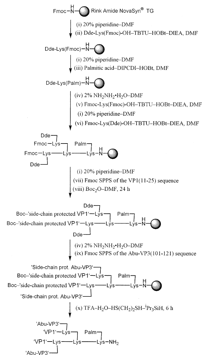
Fig. 2. Strategy of solid-phase peptide synthesis (SPPS) of MAP[VP1+VP3].
